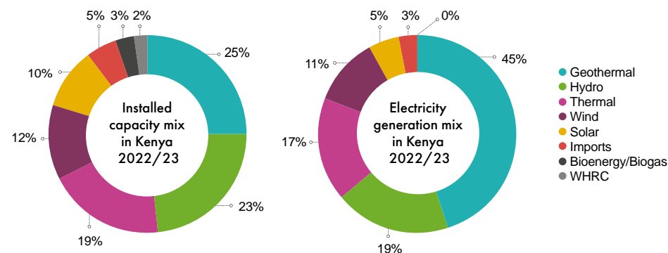
Kenya's installed capacity and generation mix, as of June 2023
