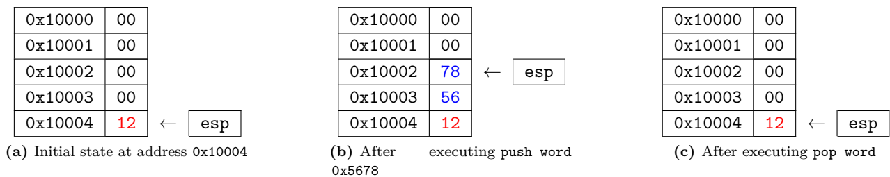
Figure 4.9.4: Stack operations
