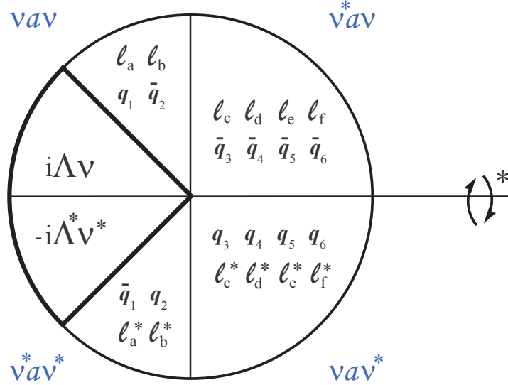
Figure 9.1: The 64-dimensional octonionic chain algebra splits into two sets of SU(3) generators of the form i\Lambda\nu and -i\Lambda^*\nu^* , six SU(3) singlets \ell_j , six triplets q_k , and their complex conjugates. These objects are sectioned off above into four quadrants according to their forms: \nu a \nu , \nu^* a \nu , \nu a \nu^* and \nu^* a \nu^* for a in the chain algebra. Transforming particles into anti-particles, and vice versa , requires only the complex conjugate * : i \mapsto -i in our formalism.
