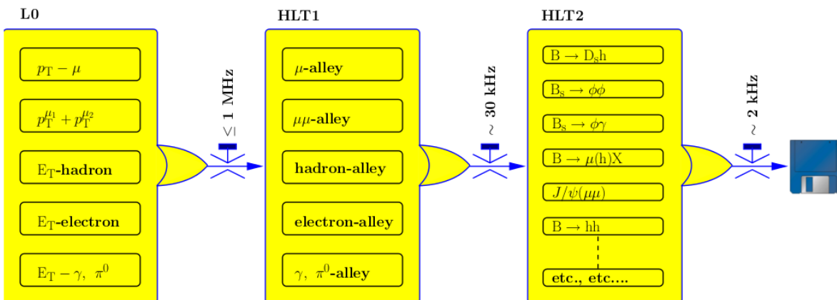
Figure 3.15: The LHCb trigger scheme.
