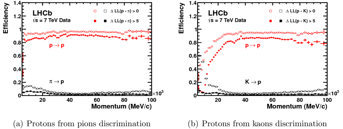
Figure 3.14: Proton identification efficiency and pion misidentification rate (left) and kaon misidentification (right) measured on data as a function of track momentum. Two different \log \mathcal{L}(p - \pi) (left) and \log \mathcal{L}(p - K) requirements have been imposed on the samples, resulting in the open and filled marker distributions, respectively.
